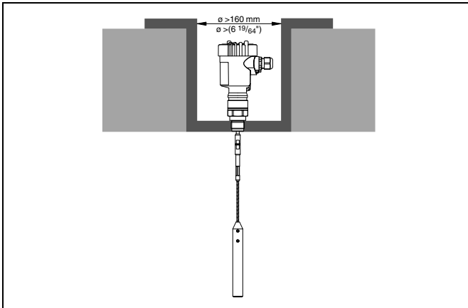
Fig. 7: Installation in concrete silo
