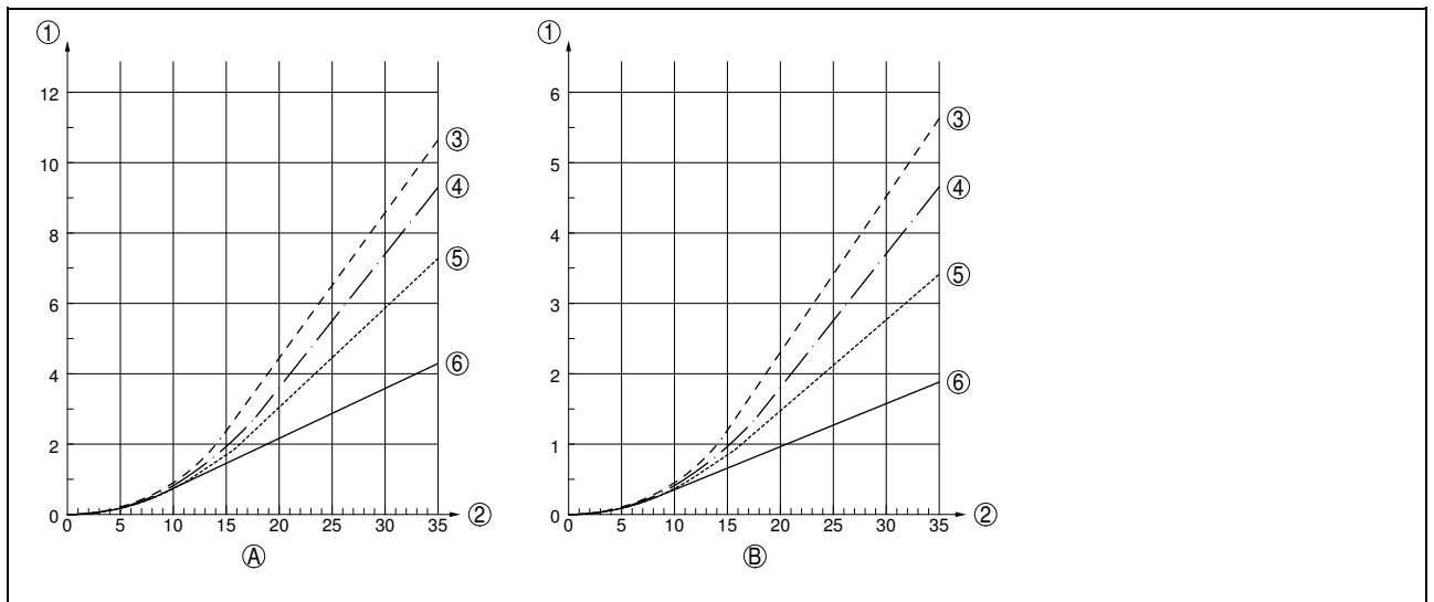
Fig. 16: Max. tensile load for VEGAFLEX 61 with cable: \varnothing 4 mm (0.157 in)
