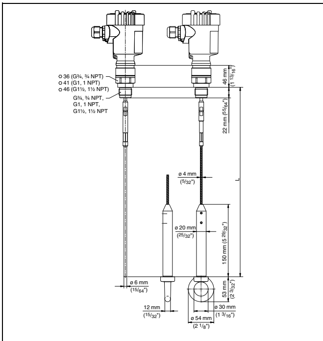
Fig. 26: VEGAFLEX 61 - cable and rod version with thread
