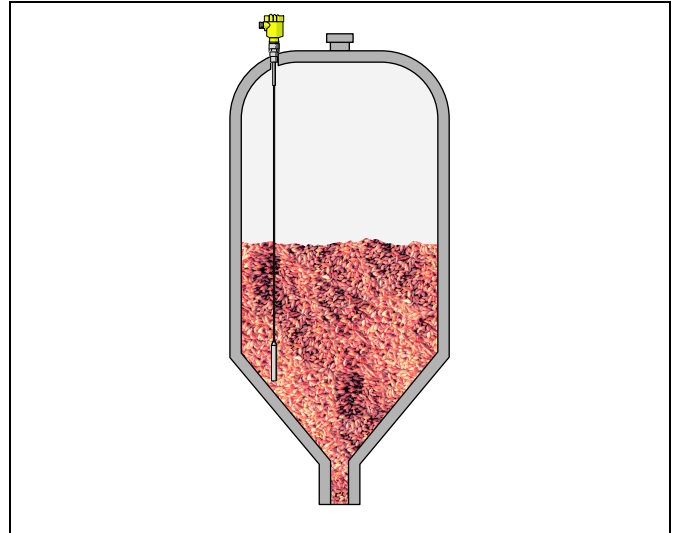
Fig. 1: Level measurement in a grain silo with VEGAFLEX 61
