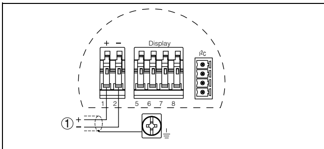
Fig. 9: Connection HART two-wire, Profibus PA, Foundation Fieldbus
