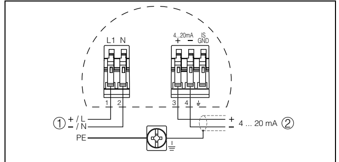
Fig. 11: Connection 4 ... 20 mA/HART four-wire
