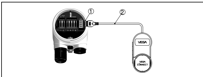
Fig. 15: External connection of the PC directly to the sensor via I²C interface
