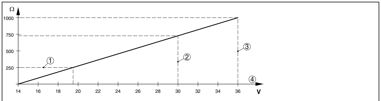
Fig. 24: Voltage diagram
