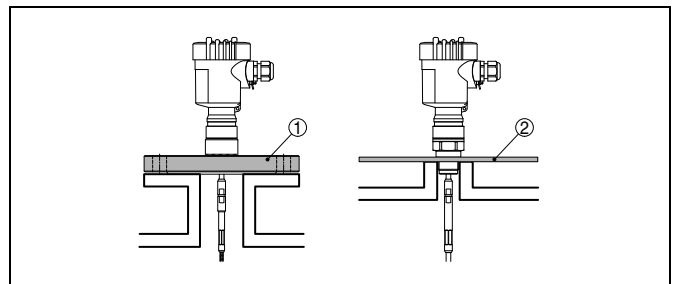
Fig. 6: Installation in plastic silo
