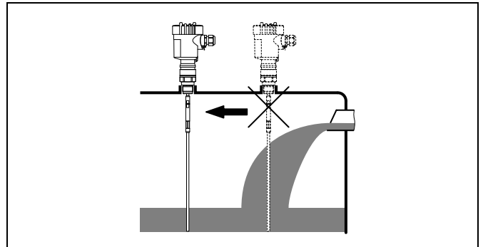
Fig. 5: Lateral load
