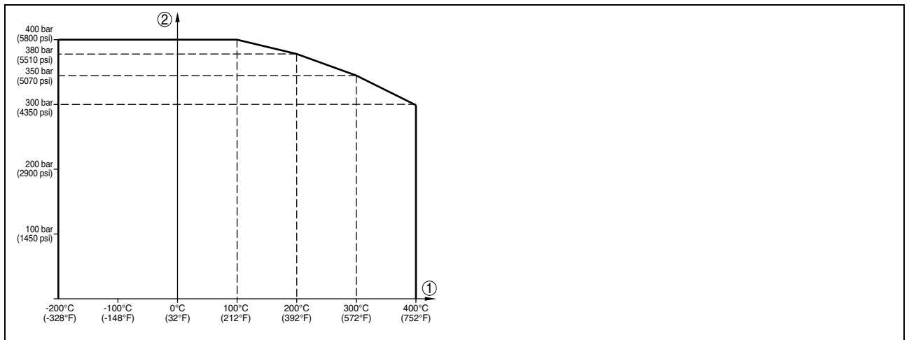
Fig. 21: Version -200 ... +400 °C (-328 ... +752 °F): dependency process pressure to product temperature
