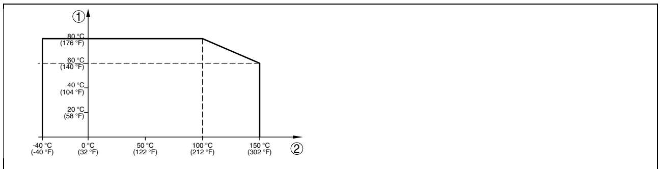
Fig. 22: Dependency ambient temperature to product temperature
