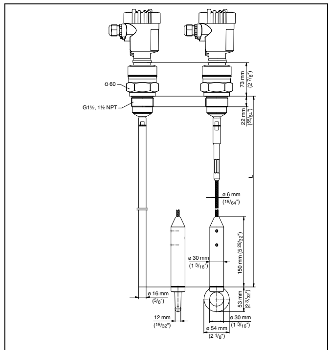
Fig. 28: VEGAFLEX 62 - cable and rod version with thread
