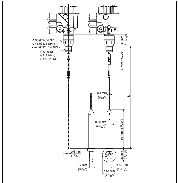
Fig. 27: VEGAFLEX 61 in cable and rod version with thread (double chamber housing)
