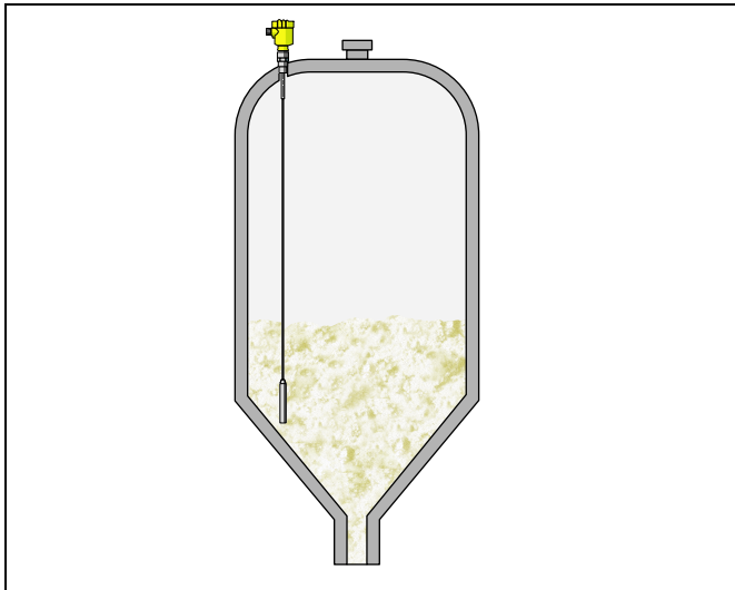
Fig. 2: Level measurement of plastic granules with VEGAFLEX 61
